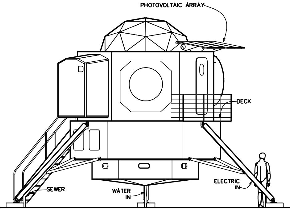
ELEVATION 2 SCALE 1/2"=1'-0"
