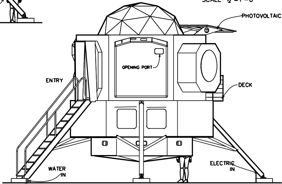
ELEVATION 1 SCALE 1/2"=1'-0"
