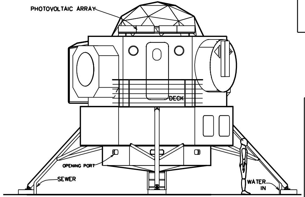
ELEVATION 3 SCALE 1/2"=1'-0"
