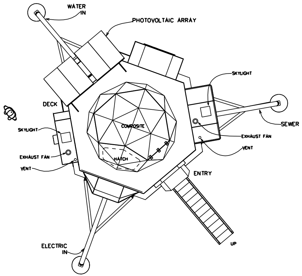
TOP VIEW - CLOSED SCALE 1/2"=1'-0"
