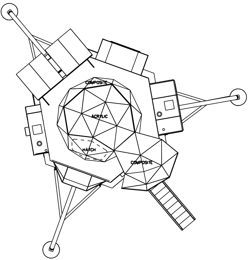
TOP VIEW - OPEN SCALE 1/2"=1'-0"
